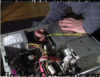
Fig. 13-5 Conector audio CD-ROM
